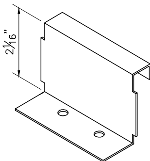
2" Fixed Mechanical Lock
