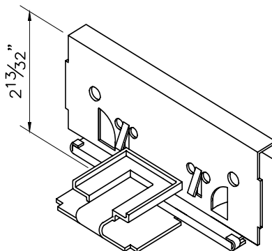
2" Floating Mechanical Lock
